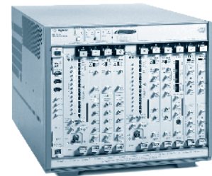
ParBERT 81250
