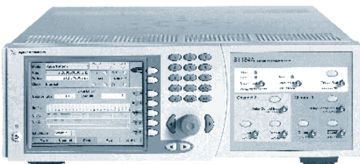
81133/34A pulse pattern generator, 3.35 GHz, dual-channel
