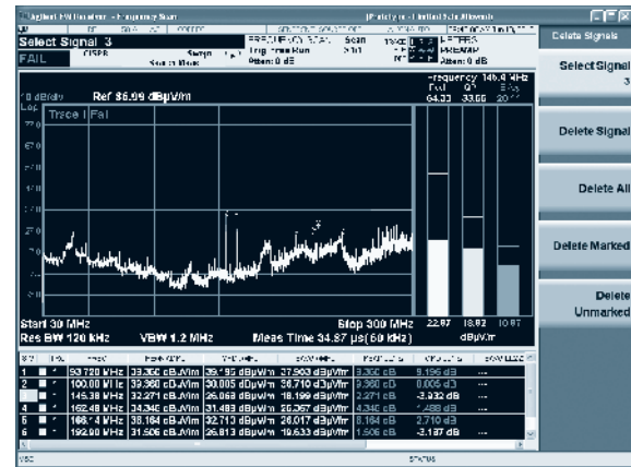
N6141A with meters and signal list
