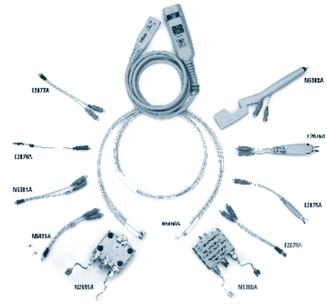
InfiniiMax II probing system with accessories
