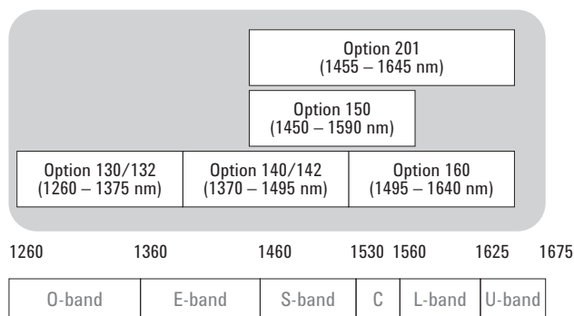
Agilent TLS-portfolio
